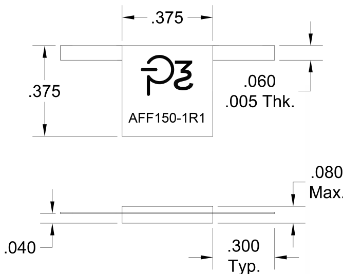
SUGGESTED MOUNTING AND TAB STRESS RELIEF METHOD
