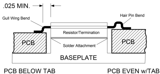
SUGGESTED MOUNTING AND TAB STRESS RELIEF METHOD
